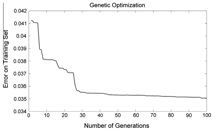
Fig. 14. Peak dataset: interval-valued training error versus number of generations in a trial for GA-IE.
