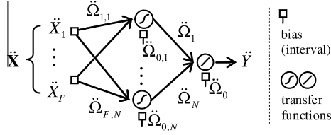
Fig. 2. The proposed MLP architecture for interval-valued data.
