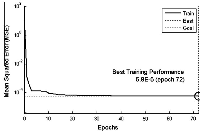
Fig. 12. Peak dataset: MSE on the training set versus the number of epochs for the conventional MLP trained with the midpoints.
