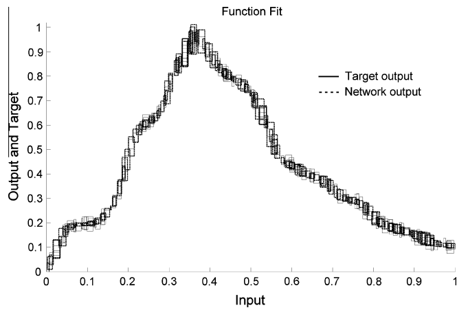
Fig. 15. Peak dataset: outputs of an interval MLP obtained in a trial of GA-IE versus the target outputs.
