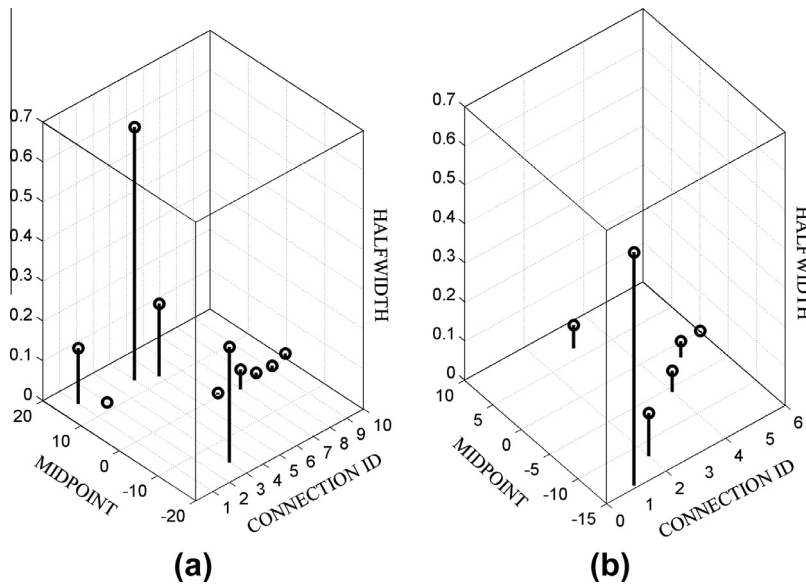
Fig. 9. Salary dataset: weights and biases in the hidden (a) and output (b) layers of an interval MLP obtained in a trial of GA-IE.
