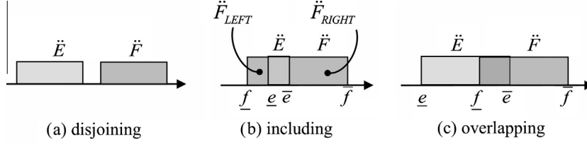
Fig. 5. Types of intervals: (a) disjoining; (b) including; and (c) overlapping.
