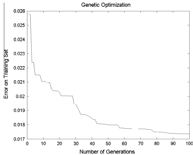
Fig. 13. Peak dataset: numeric-valued training error versus number of generations in a trial for GA-NE.
