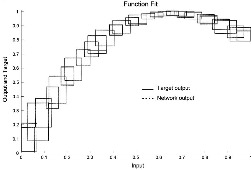
Fig. 10. Salary dataset: outputs of an interval MLP obtained in a trial of GA-IE versus the target outputs.
