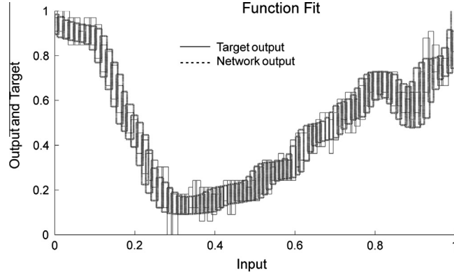
Fig. 19. The Heart dataset: outputs of an interval MLP obtained in a trial of GA-IE versus the target output.
