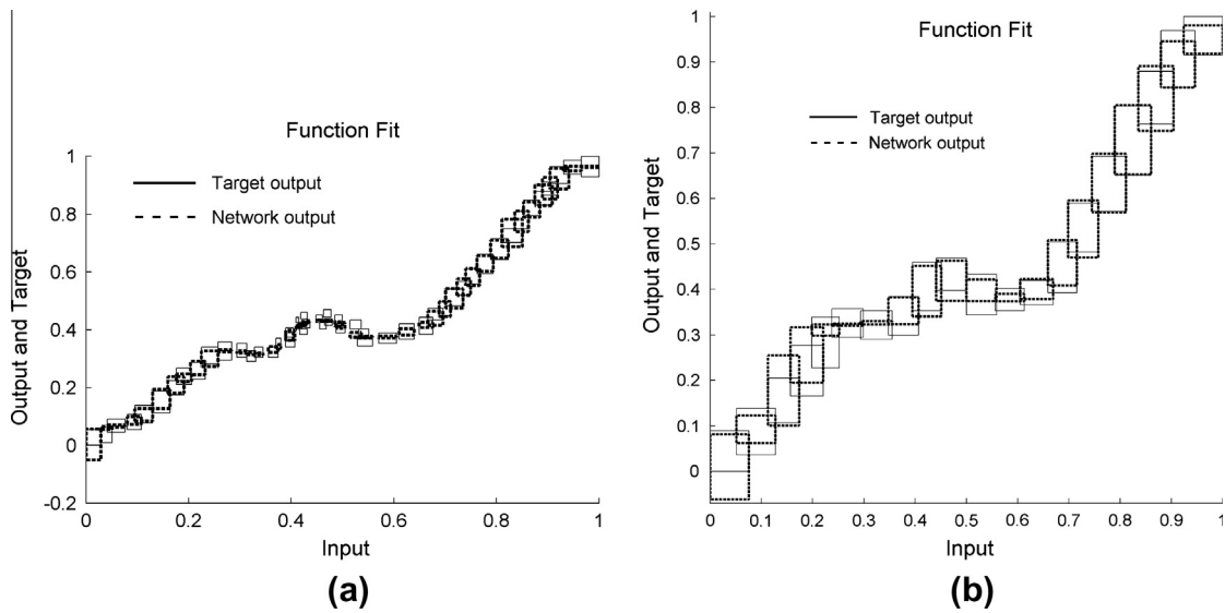
Fig. 17. Outputs of an interval MLP obtained in a trial of GA-IE versus the target output: (a) Micro-Spread dataset and (b) Macro-Spread dataset.
