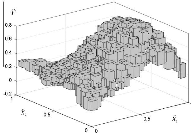
Fig. 21. Wave dataset: a high resolution mapping of an interval MLP obtained in a trial of GA-IE.
