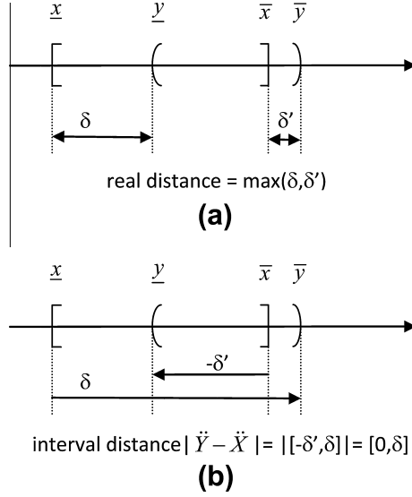
Fig. 1. Example of computation of real distance (a) and interval distance (b).
