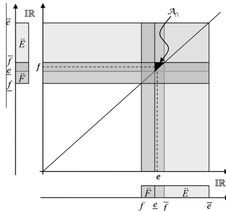
Fig. 6. An example of the area \mathcal{A}_\cap of the Cartesian product in the Overlapping scenario.
