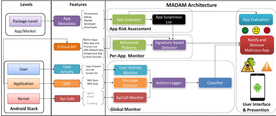
Figure 1. Architecture of MADAM
