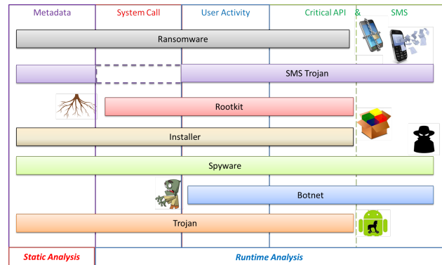
Figure 2. Relevant features for the Detection of the Seven Malware Behavioral Classes
