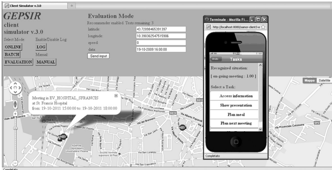
Fig. 24. The auxiliary web application to evaluate the recommender.
