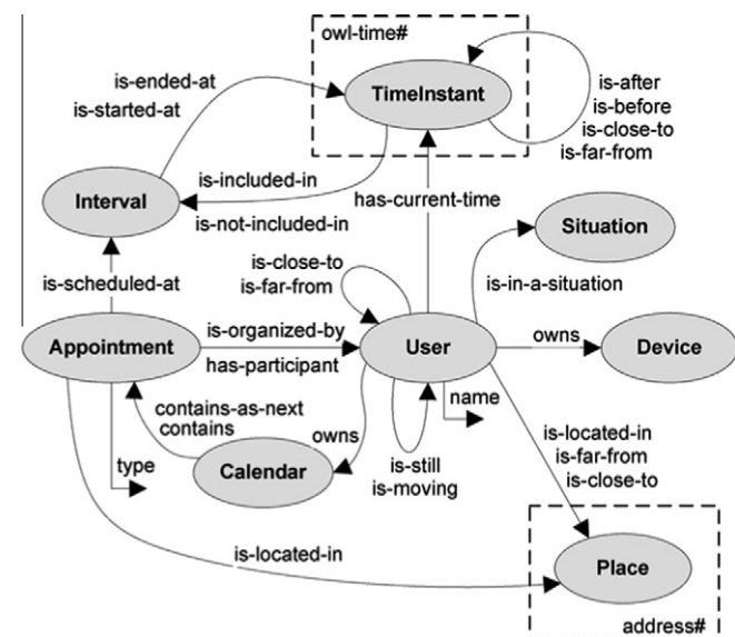
Fig. 5. The upper context ontology.
