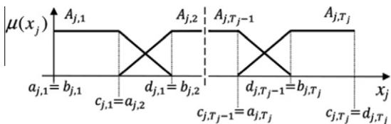
Fig. 17. A generic partition of a linguistic variable.
