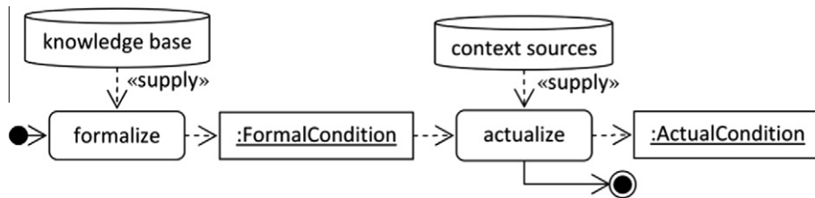
Fig. 15. The formalization-actualization process.
