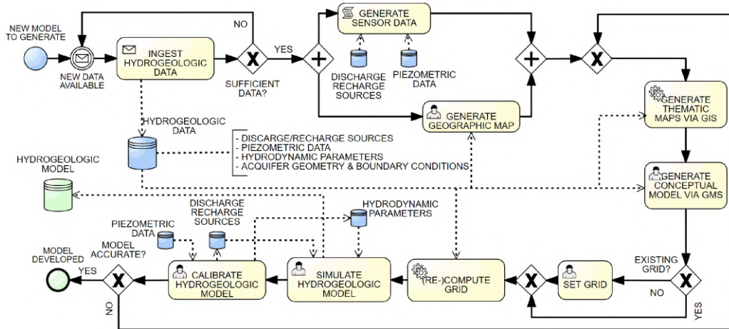
Fig. 1. BPMN workflow of groundwater Process-driven Modeling.
