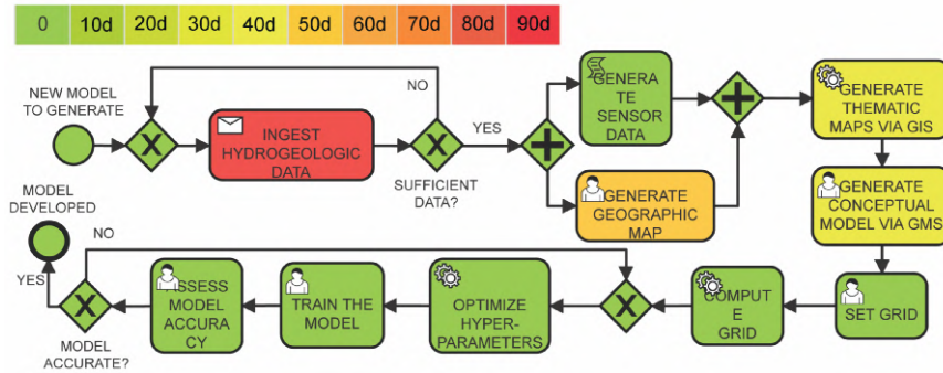
Fig. 6. Heatmap based on durations for Data-driven Modeling
