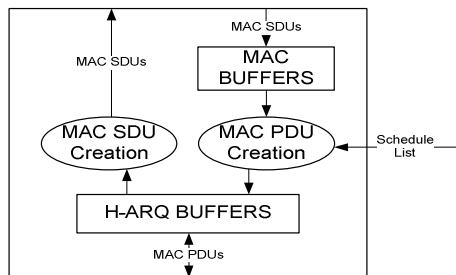
Figure 5: MAC packet flows.
