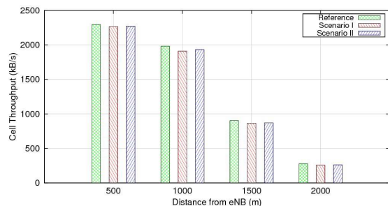
Figure 10 - Cell Throughput for Scenario I and Scenario II compared against theoretical reference throughput.
