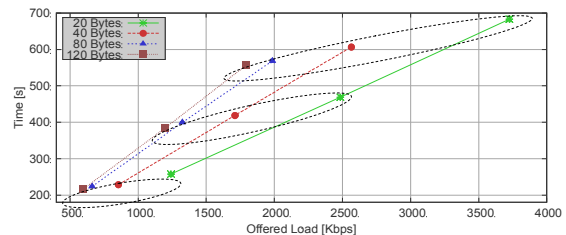
Figure 13: Execution time with varying offered load.
