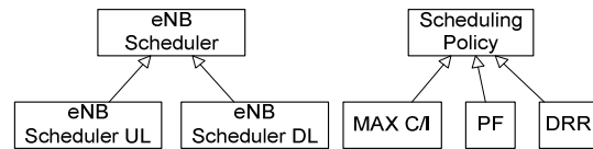
Figure 9: eNB schedulers and Sch. Policy hierarchy.
