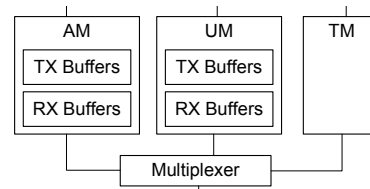
Figure 4: RLC module representation.
