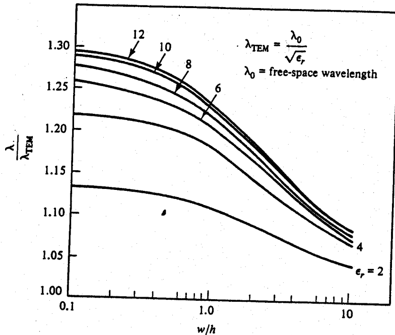
Figure 6-1-2 shows the normalized wavelength of a microstrip line versus w/h
