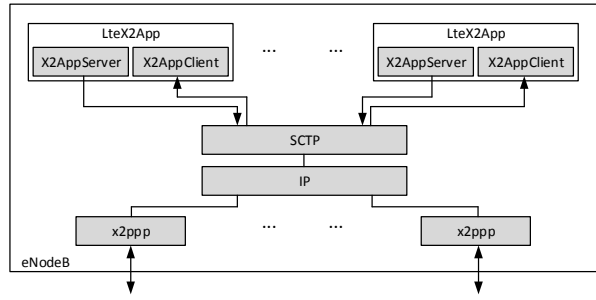
Fig. 3. Layering of the X2 interface
