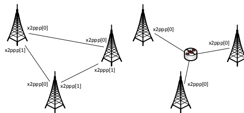
Fig. 4. Full mesh (left) and star (right) topologies
