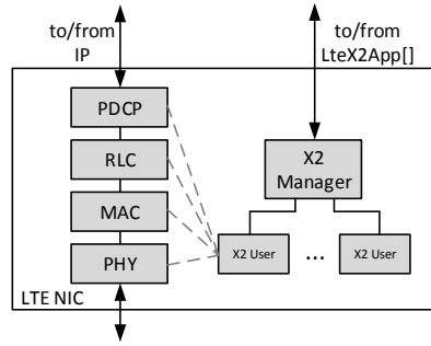
Fig. 6. Interface between LTE NIC and X2 in the eNB
